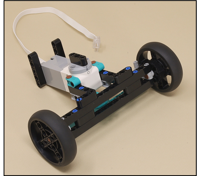
Ackerman Steering
