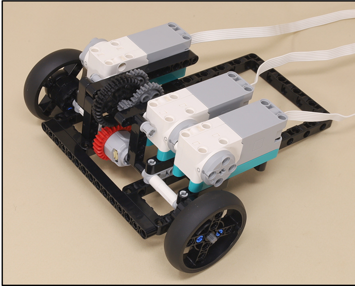
3 Motor Drive
