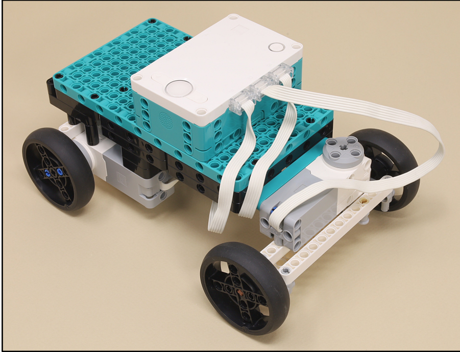
Pickup Truck Chassis
